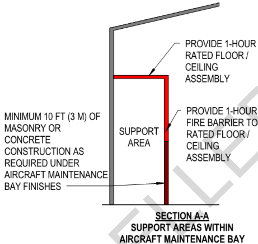
Figure 3-1-1: Internal Fire Rated Separations
